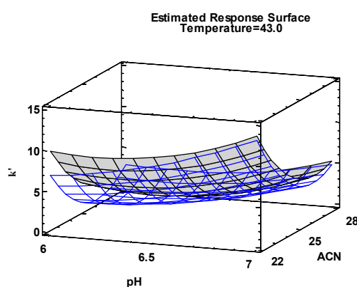
Figure 4. Overlaid response surfaces of AZT and EAIE. The blue and grey coloured surfaces represent the individual response surfaces of EAIE and AZT respectively.
