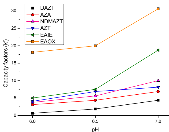
Figure 2. Effect of buffer pH on capacity factors of components of the working mixture.
