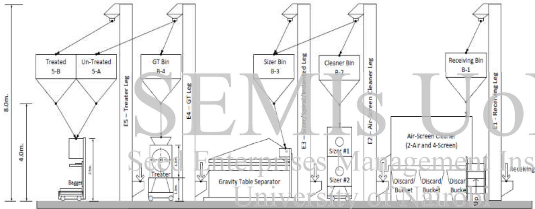
Flow Diagram for Seed Cleaning Operation
