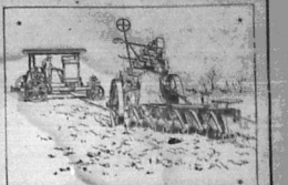
The Ploughing with McLAREN'S PATENT MOTOR CABLE TACKLE (Double Engine System).
