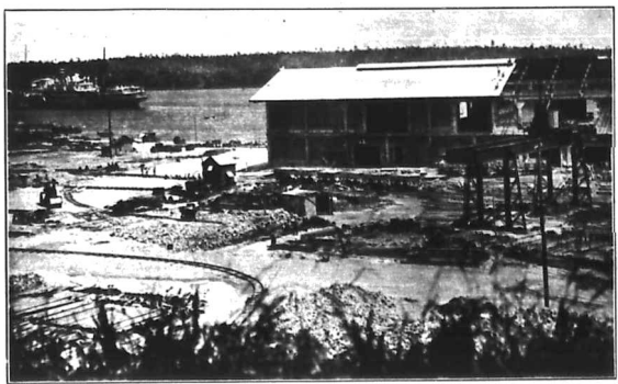
Construction work at Kilindini Harbour Works, showing the large crane and building completion. Photo: P. P. P.
