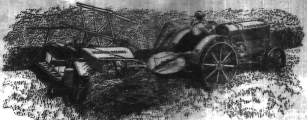
A power take-off, its mechanism being operated by the lower shaft of the McCormick-Deering tractor.
