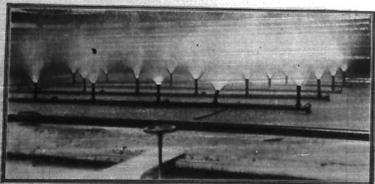
The spray tank for lowering the temperature of the circulating water cooling system.
