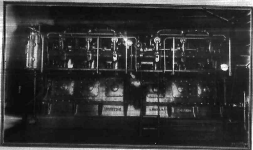
One of the three Ruston and Hornsby, oil-fired, direct injection, cold starting six cylinder oil engines, in each of which is coupled a 200 kilowatt alternator of the Electric Construction Co. Ltd., generating at a pressure of 8,500 volts.
