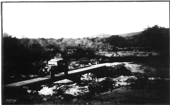
The new bridge over the Tana River. This bridge is one of the many links between the Capital and the Port and the old structures were a constant source of trouble. The story of the Causeway and the Tana Bridge is told in this issue by Mr. L. D. Graham-Fox, Hon. Secretary of the R.E.A.A. to whom this "Standard" is indebted for the photographs.
