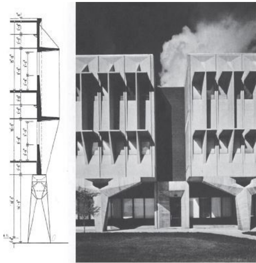
Fig 2.32. Section and image of brise soleil in design by Mark Bruere who was inspired by Le Corbusier Source: Yao (2021)
