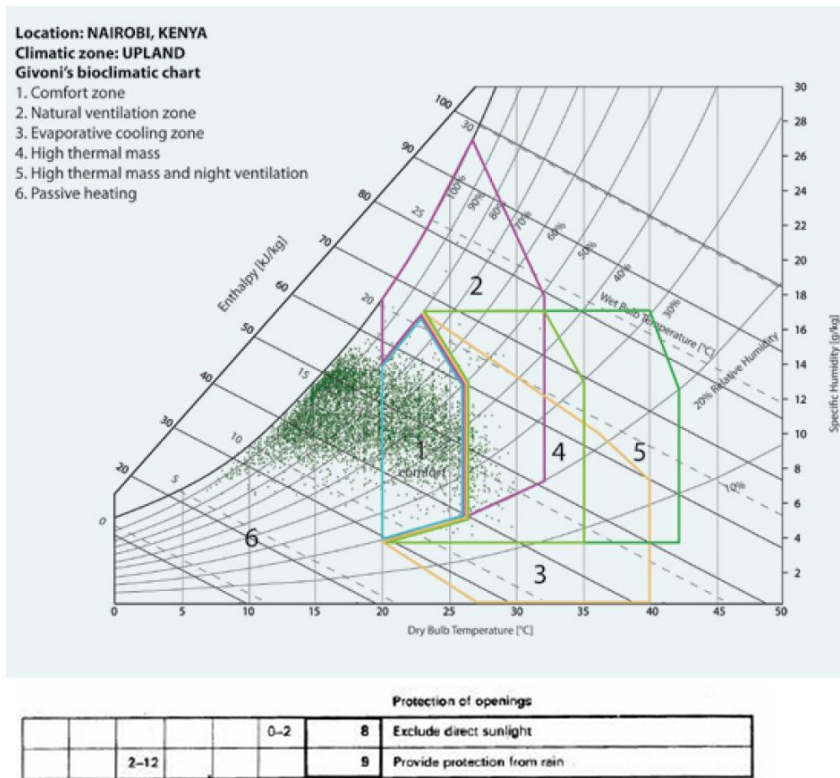
Fig4.3. Psychrometric Chart and Mahoney table recommendations for Nairobi.
