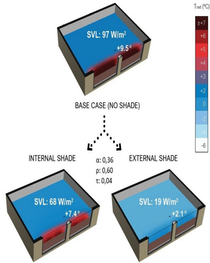
Fig2.47. Simulation of internal temperature calculations in a building when using internal and external shading devices.
