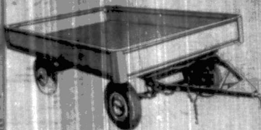
NATAL TRAILER This trailer is carried on high-tensile steel and equipped with non-slippery springs, full shock absorber system, ball-bearing axles and carrying frames, strong tie-downs, and 1000 lb. capacity bumper. Size 11 ft. x 6 ft.
