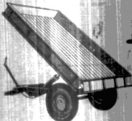
NELKOR'S TRAILER 3-Ton All-steel hydraulic tipping trailer for use with Tractor equipped with Hydraulic Power.
