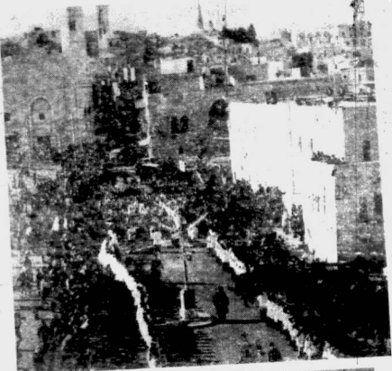
Above: The large crater Langrenus as photographed from an altitude of 3,625 miles as Apollo 8 orbited the Moon. Langrenus is about 85 miles in diameter. Left: The procession formed in Manger Square, Bethlehem, on Christmas Eve before being led to the Church of the Nativity by the Latin Patriarch, Msgr. Alberto Gorio. A strong contingent of troops was on duty in the Holy City in view of outbreaks of violence during the Christmas holidays.
