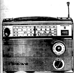
SONY TR-814 Powerful 8-transistor, 3-band radio which has wide frequency coverage providing international and domestic shortwave bands (MW; SW 150-50m & 50-16m), handsomely designed cabinet with fine tuning and V speaker. Uses 4 flashlight batteries (size D).
