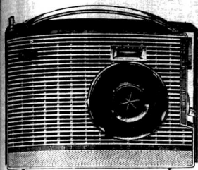
SONY TR-814 Powerful 8-transistor, 3-band radio which has wide frequency coverage providing international and domestic shortwave bands (MW; SW 150-50m & 50-16m), handsomely designed cabinet with fine tuning and V speaker. Uses 4 flashlight batteries (size D).
