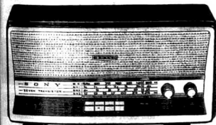
SONY TR-719 4-Band (MW; 3-SW bands 200-11.5m), all transistor home radio with fine tuning and piano style push buttons. Beautifully designed modern mahogany finished cabinet—performs brilliantly where other radios fail and adds distinction to any surrounding! Uses 4 flashlight batteries (size D). An important member of your family.
