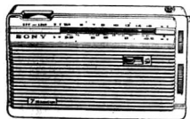
SONY TR-716 2-band portable with dial lamp and fine tuning control. Gives excellent performance with amazingly high sensitivity and selectivity. SONY TR-716B (MW; SW 77-25m); SONY TR-716Y (MW; SW 50-16m). Uses two economical flashlight batteries (size C).
