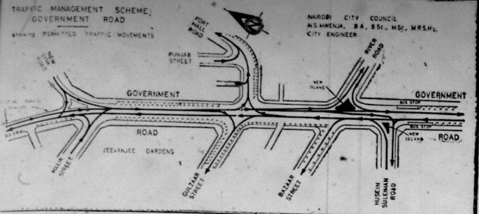
Alterations are to be made to Government Road in Nairobi to reduce the danger of accidents and speed the flow of traffic. The above diagram shows the new routes for traffic which are explained on the right.
