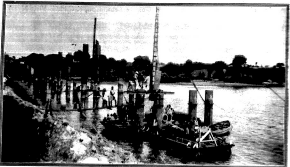
Reconstruction of old railway bridge at Mwarua, built in 1897, and now being used to carry electricity for line for water supply to Mwarua, Kenya.
