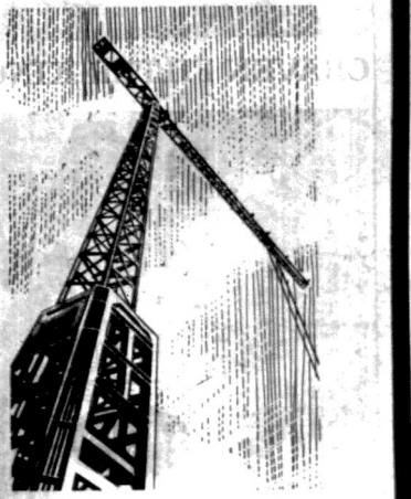
This Tower Crane was made by Pearson Tower Cranes Ltd. using R.H.S. for both the mast and jib. R.H.S. have been used in this structure because of their greater efficiency in compression and excellent torsional resistance. The crane, though lighter than a conventional one, is able to carry heavier loads.
