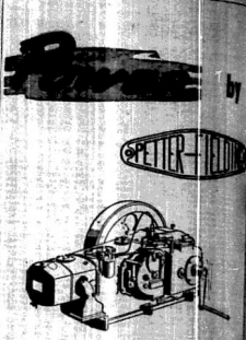
PETTER-FIELDING HORIZONTAL ENGINE EA 21/2 I.H.P. AT 500.50 FL.P.M.
