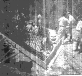
An aqueduct under construction to carry the furrow over a gully. In the top picture, workers use pneumatic drills to get through a hard rock section of the furrow's alignment.
