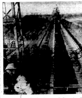
New Repco 2000 high-grade iron ore recently discovered in the national consortium. The ore dump above the London model (left) are 100 and distributed by two conveyor systems, which return them to the pneumatic-transported load, (right) in the tunnel setting in the rail cars below.
