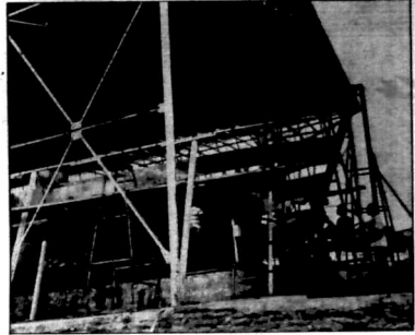
Steady progress is being made in the Mombasa dockyard of the East African Railways and Harbours in the construction of the first all-steel pier just to be built above. The pier is to take ships with three masts on the starboard side completed. Right: Trains overnight (left) Kenya connects some of the territories on the job of the SGR rail.
