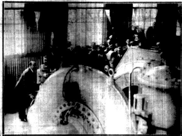
His Excellency the Acting Governor, Mr. H. M. M. Moore, sitting in motor car on the 2,000 horse power turbines at the new power station on the Tana River of the East African Power and Lighting Company, on Monday. This is the first step in a larger scheme for making use of the power resources of the Tana and Maragua rivers.
