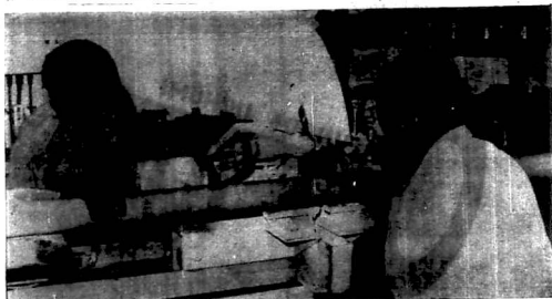
Production of P.V.C. pipes at the Falim Plastics factory in Nairobi is fully automatic. Here two operators watch as the pipe is cut into 500 lengths on the extrusion line.
