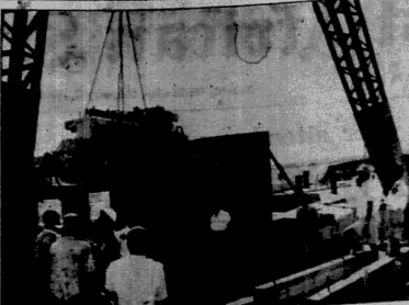
The engine is lowered into the new 100-ton passenger launch under construction at the East African Railway and Harbours Marine Works at Kisumu.
