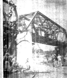
Bottom.—Sixth Bridge ready for use. The two new concrete spans, each weighing 20 tons, can be seen. They are supported by light steel trusses on reinforced concrete abutments. The bridge is the first of the type to be built in Burma since the Japanese started their operations in 1942. The reason was a flood, but after the bridge was repaired there was no more trouble. Top left.—The head work being done on Pyawbun Bridge where the new spans (on the left of the picture) rest on the bomb-damaged pier near the old bridge. Top right.—Sapper Edd, Montgomery, Temporary Officer of the 21st (Engineers) Battalion East African Engineers, at work.
