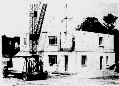
PICTURED above is the premises of the new building at Nairobi, which is being built by the new method. It is a 100-foot long and 40-foot wide building, built with precast concrete slabs.
