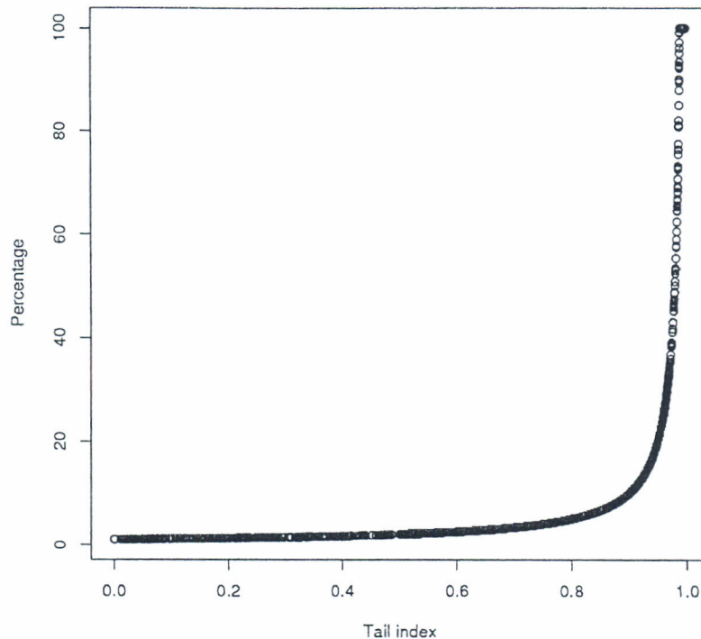
Figure 5: The proposed re-insurance proportions in relation to the tail index
