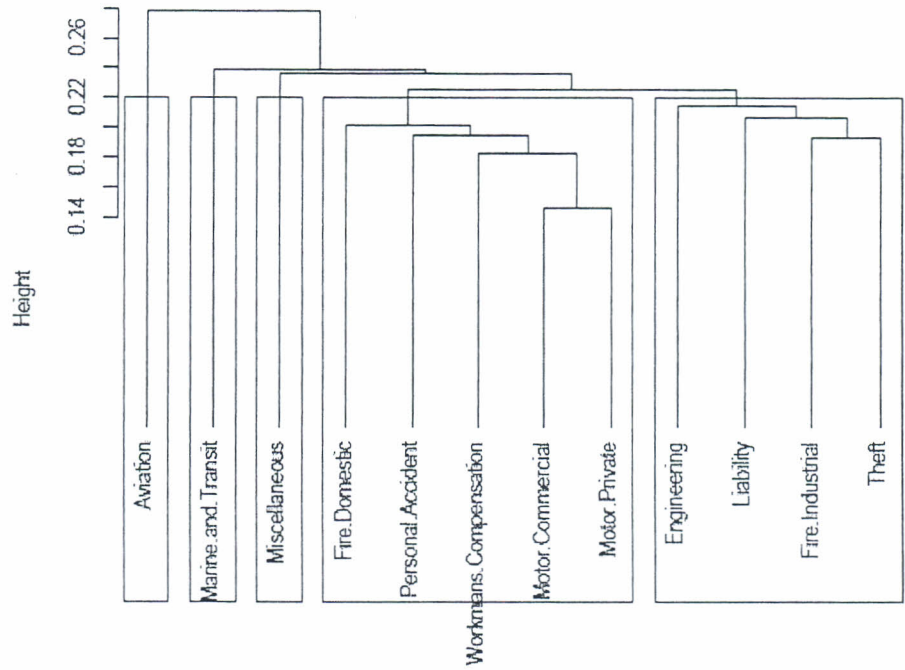
Figure 3: The general insurance classes clustered by the Euclidean distances for the Kendall's tau
