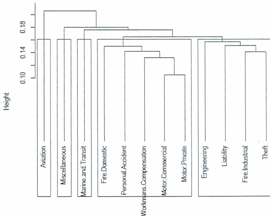
Figure 2: The general insurance classes clustered by the Euclidean distances for the Tail index
