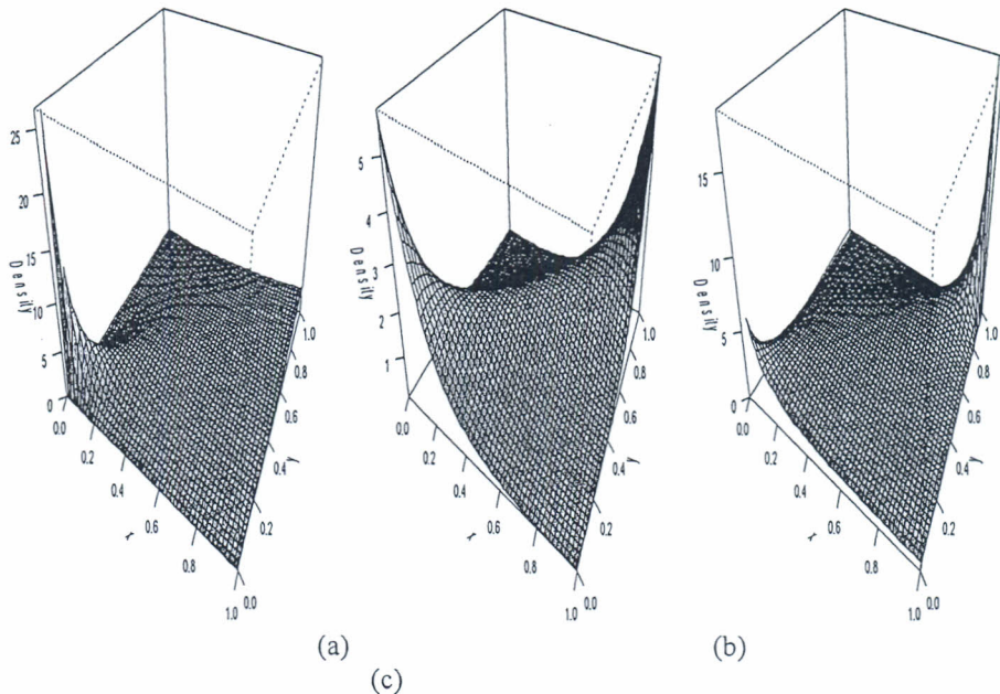
Figure 1: Perspective plots for the (a) Clayton, (b) Frank and (c) Gumbel copulas
