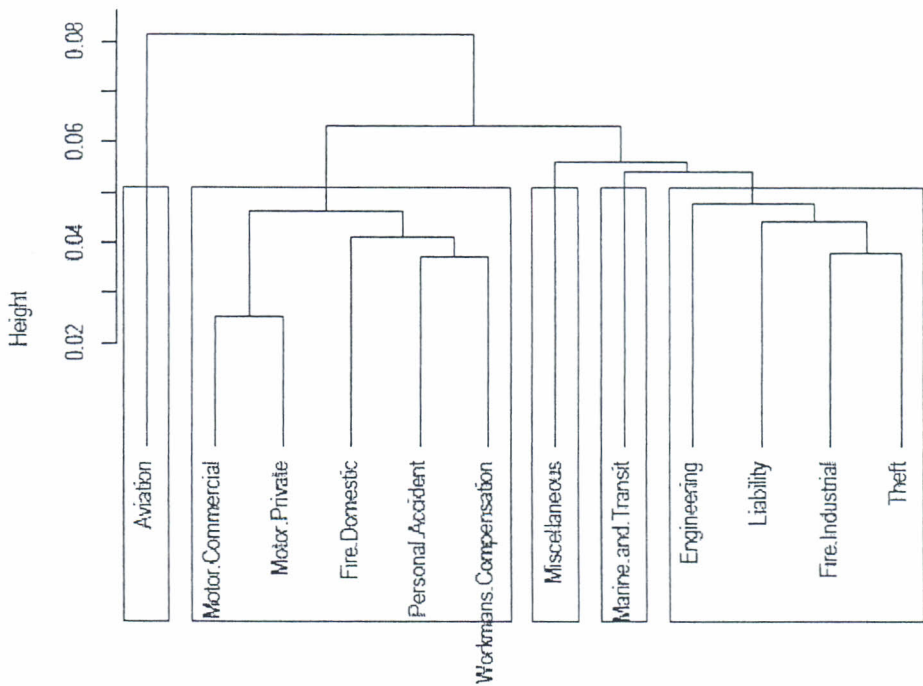
Figure 4: The general insurance classes clustered by the Euclidean distances for the Spearman's rho
