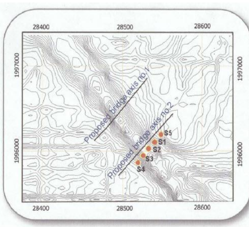
Figure 6-15: Location of soil sampling
