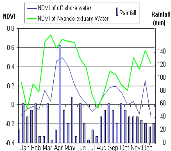
Figure 4- 4: NDVI Multi-temporal behavior of the off Shore water and water from Nyando Estuary in 2007 in the Lake Victoria.
