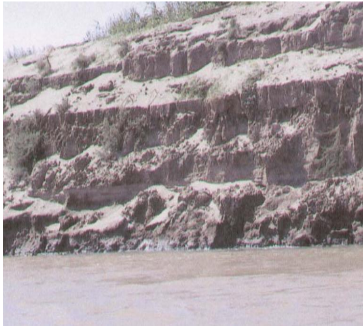
Figure 3- 7: Bank erosion – Sliding failure type in Northern State (Karima – Dongla Reach)
