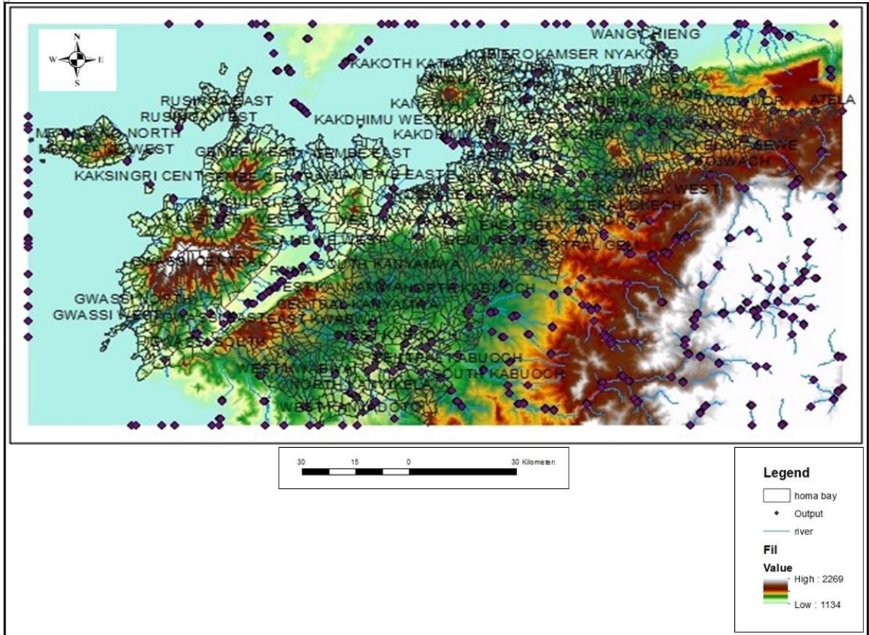
Figure 3.6: Rivers and streams in Homa Bay County
