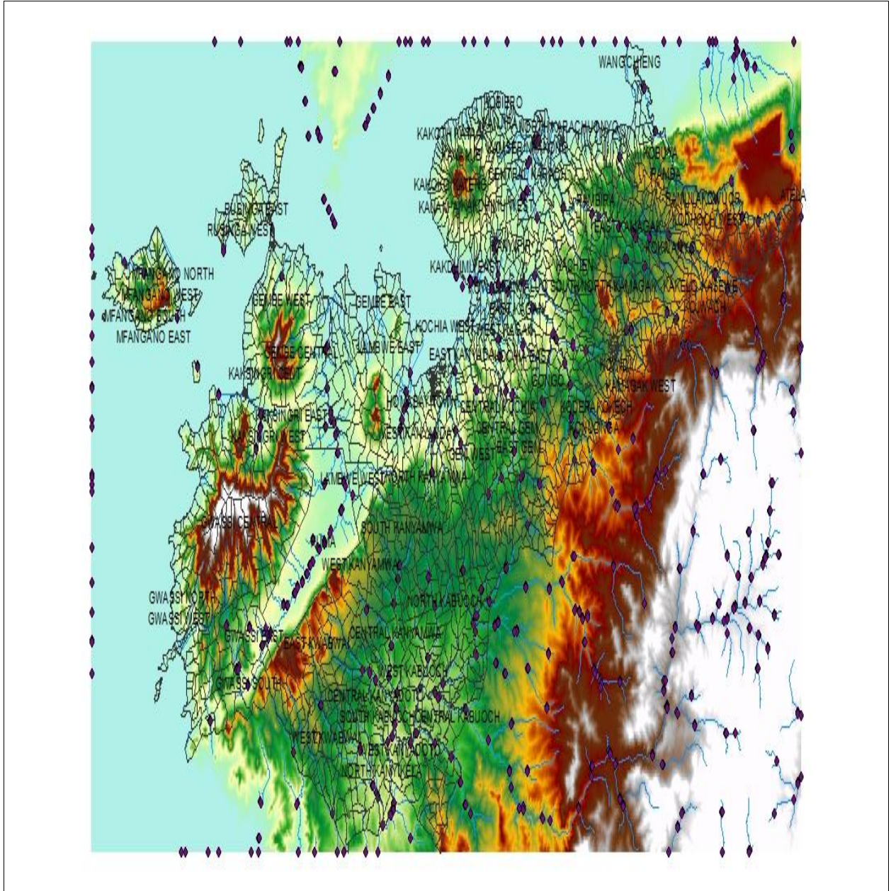
Figure 3.5: Rivers flowing through Homa Bay County
