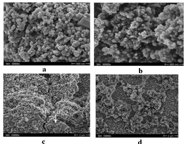
Figure 5. SEM images of TiO_2/Nb_2O_5 composite films (a) 5.5 μm film showing uniform coating before annealing, (b) 12.0 μm film before annealing showing agglomeration (c) 12.0 μm film showing micro cracks after annealing at 450.0°C and (d) 5.5 μm film showing absence of micro cracks after annealing
