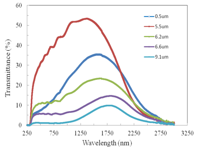
Figure 4. Variation of transmittance with wavelength in TiO_2/Nb_2O_5 composite films of various thicknesses deposited at 35.0 V for 90.0s.
