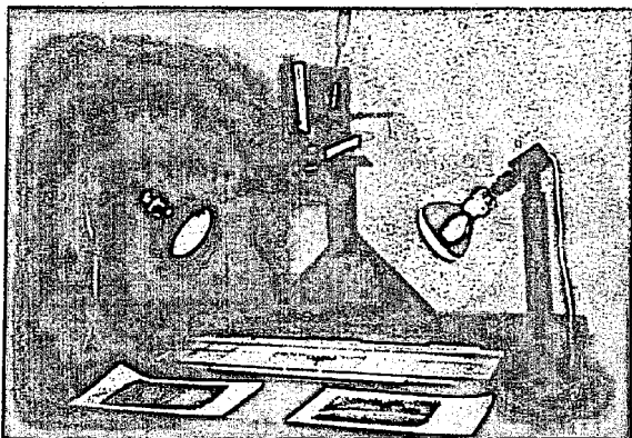
Figure 27. Animation stand. The Canon 814 camera is fixed in one position and equipped with a close-up lens, single frame cable release, and black paper reflecting shield. A long piece of glass from a louver window holds the material flat. Lights are ordinary 150 watt household flood lamps.
