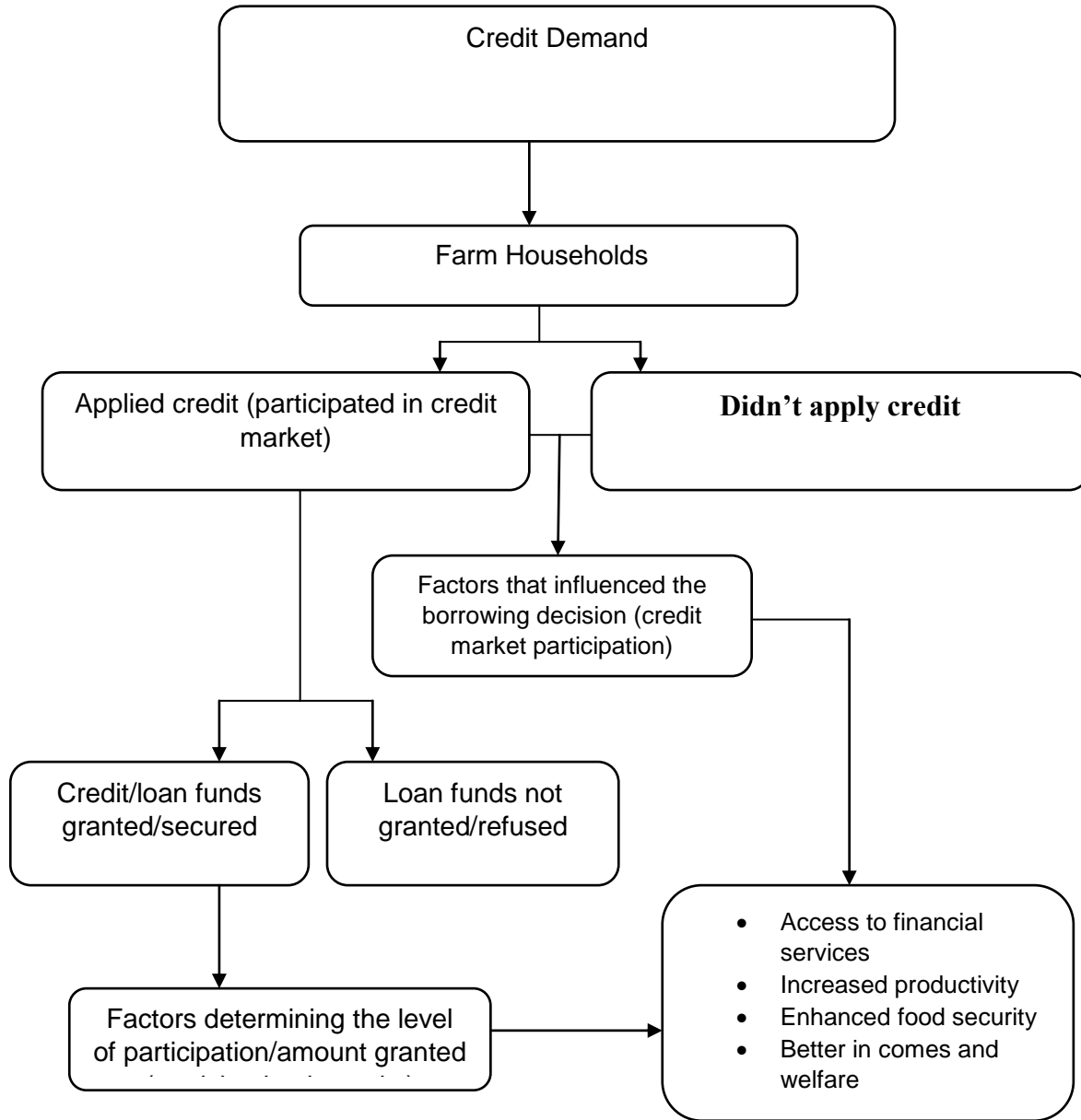
Figure 2: Conceptual Framework
