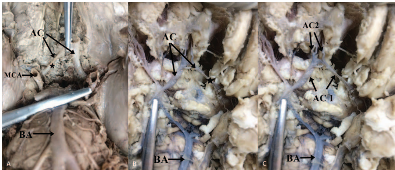
Fig. 1 (A) Unilateral hypoplasia of A1 segment of the left anterior cerebral artery. Note the asterisk which highlights the variant artery. (B) Unilateral hypoplasia of A1 segment right anterior cerebral artery. Note the asterisk which highlights the variant segment. (C) Unilateral hypoplasia of A2 segment of anterior cerebral artery 2. Abbreviations: AC 1, first part of anterior cerebral; BA, basilar artery; MCA, middle cerebral artery.
