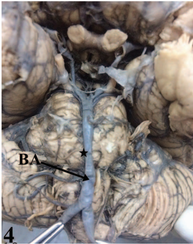
Fig. 4 Basilar artery hypoplasia.
