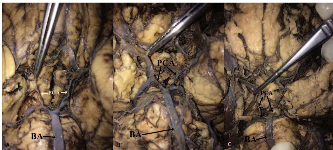
Fig. 3 (A) Bilateral hypoplasia of posterior communicating artery. (B) Unilateral hypoplasia of the right posterior communicating artery. (C) Unilateral hypoplasia of the left posterior communicating artery. Abbreviation: BA, basilar artery.
