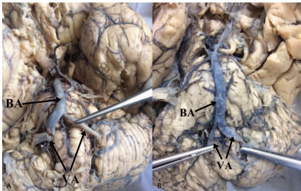
Fig. 5 (A) Mild left vertebral artery hypoplasia. (B) Mild right vertebral artery hypoplasia. Abbreviations: BA, basilar artery.
