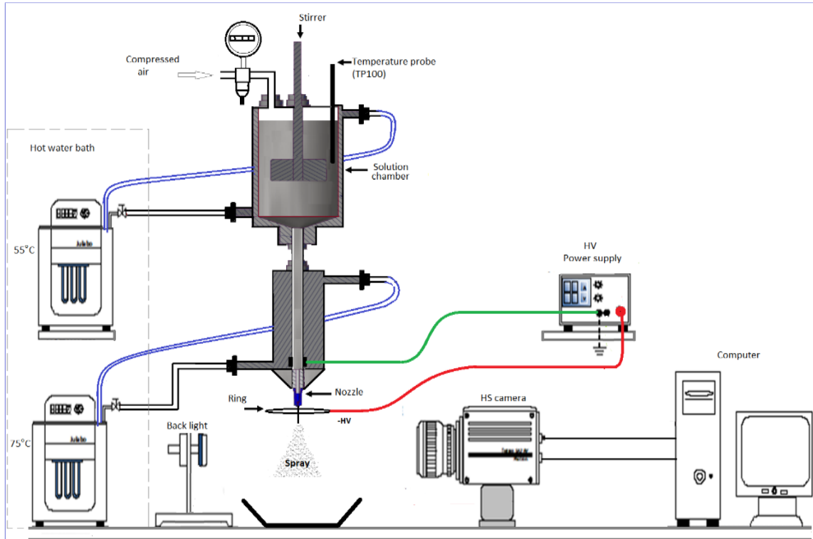
Figure 3.1: Experiment Setup
