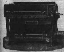
MAGAHEY DOUBLE-ACTION SINGLE ROLLER COTTON GINN, For Power 40 inches wide.
