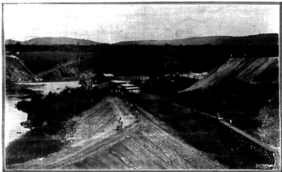
The approach to the bridge from the left side. The 75 feet embankment on the extreme right gives an impression of the level at which the railway will cross the river. The embankment in the center will carry the road on to the bridge at a height of 50 feet above the water.
