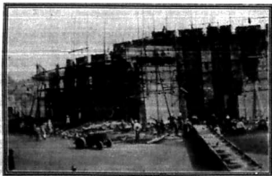
Moving the biggest girder in East Africa. One of the huge 15 ton parts of the Salisbury Bridge, the link between Mombasa and the mainland. The bridge is now dismantled since a narrow-gauge was built and the girder is being used to support the railway of Nairobi and 1,000 mile Thika. The picture shows the girder being moved by the Express Transport Co., Nairobi, who built a special carrier for the job.
