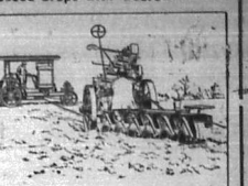
The Ploughing with McLAREN'S PATENT MOTOR GEARL TACKLE (Double Engine System).
