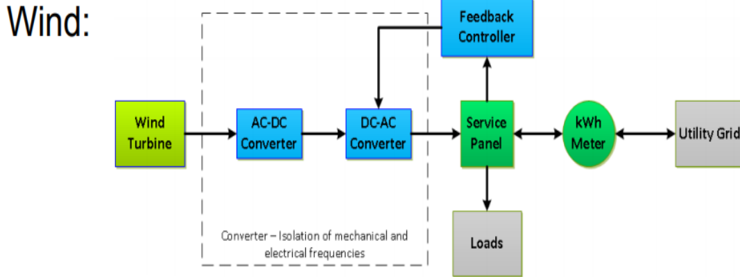
Figure 2.1: Integrating Wind Power to the Electrical Grid [1]
