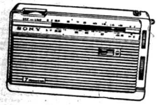
SONY TR-716 2-band portable with dial lamp and fine tuning control. Gives excellent performance with amazingly high sensitivity and selectivity. SONY TR-716B (MW; SW 77-25m); SONY TR-716Y (MW; SW 50-16m). Uses two economical flashlight batteries (size C). Shs. 320/-
