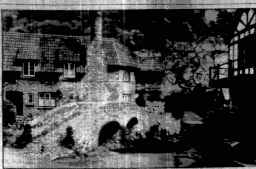
A brickworker to protect the foundations of the old pass here being built into the new bridge. The structure has been newly erected and is a favourite subject for artists.
