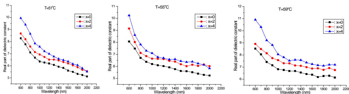
Figure 5. Real part of dielectric constant against wavelength at different substrate temperatures.
