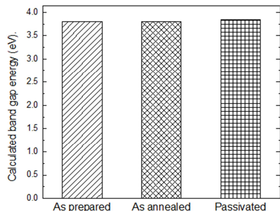
Figure 10. Calculated band gap energy for the as prepared, annealed and passivated F: SnO 2 thin films.
