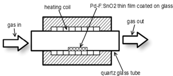
Figure 2. Horizontal tube furnace for annealing and passivation.
