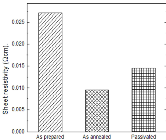
Figure 13. Sheet resistivity for the as prepared, annealed and passivated Pd: SnO 2 thin films.
