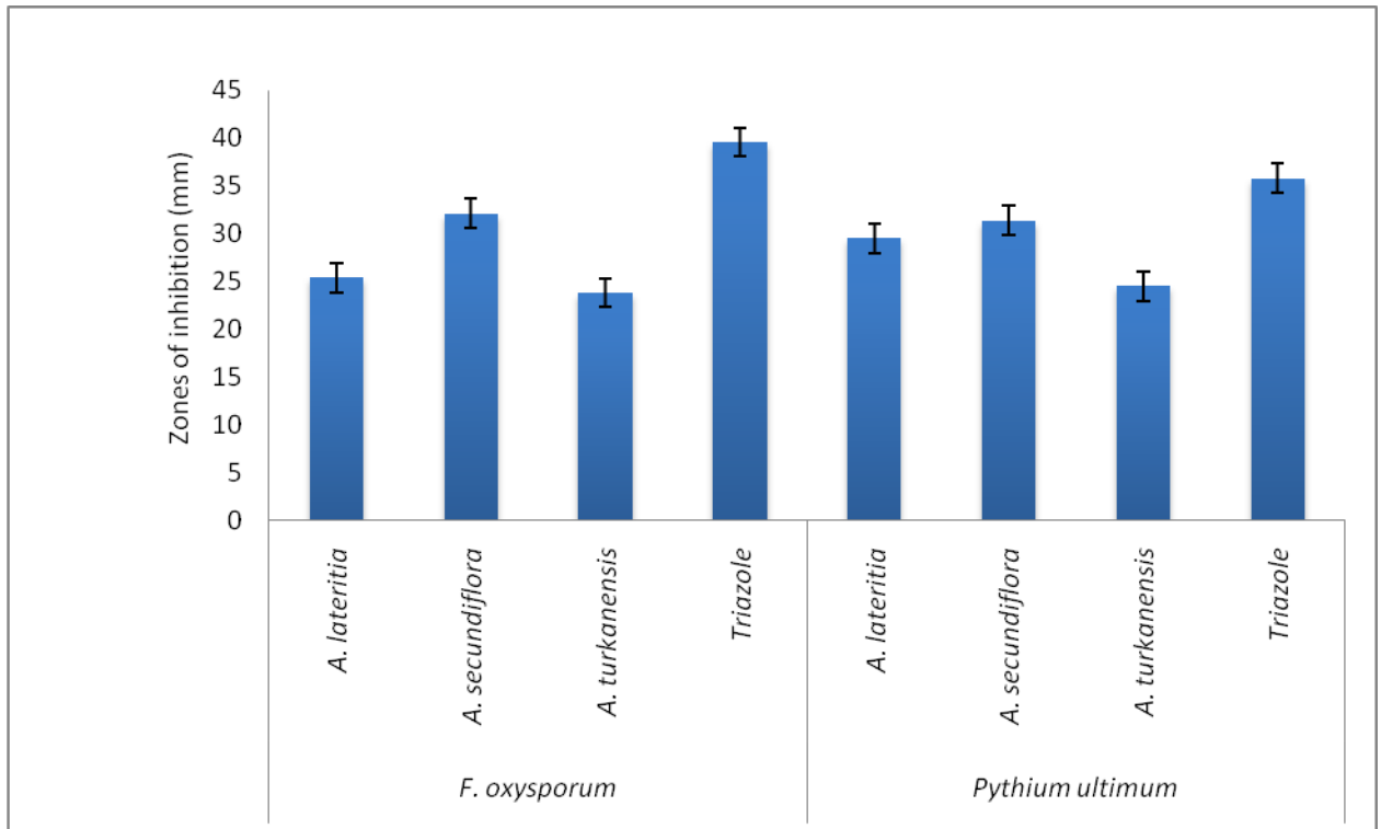
Figure 9: Mean inhibition (mm) of growth of F. oxysporum and P. ultimum by crude extracts of different Aloe species
