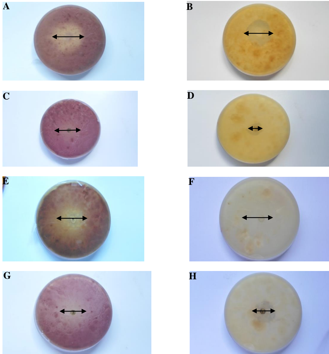
Figure 8: Zones of inhibition (mm) formed by crude extracts of Aloe species and the standard fungicide Triazole on F. oxysporum and P. ultimum after 10 days of incubation Triazole on F. oxysporum (A) and P. ultimum (B) at 50mg/100 \mu l; crude extract of A. turkanensis on F. oxysporum (C) and P. ultimum (D) at 25mg/100 \mu l; crude extract of A. secundiflora on F. oxysporum (E) and P. ultimum (F) at 100mg/100 \mu l; Crude extract of A. lateritia on F. oxysporum (G) and P. ultimum (H) at 100mg/100 \mu l.
