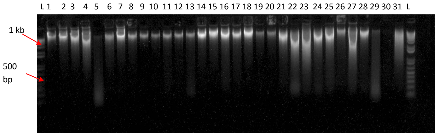
Figure 3: DNA profile – Agarose gel electrophoresis of Aloe DNA Key: Lane 1- 31: Aloe accessions as shown in Table 1, L: Ladder
