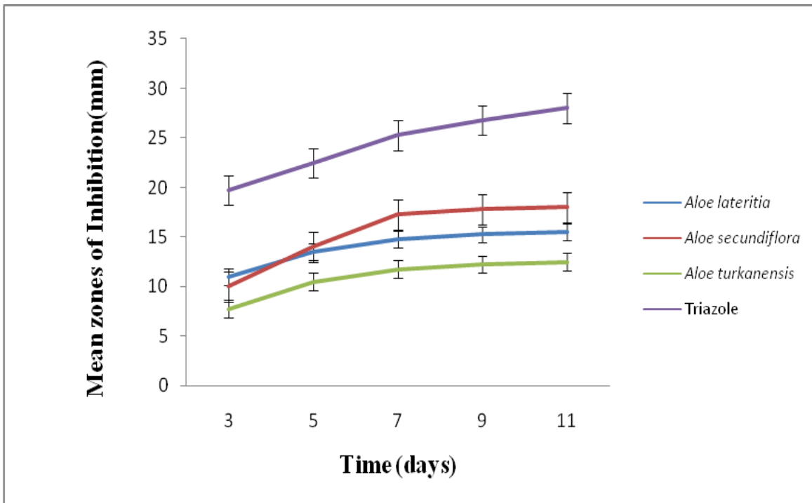
Figure 12: Mean inhibition (mm) of growth of F. oxysporum (A) and P. ultimum (B) by crude extracts of different Aloe species at a 25mg/100 \mu l concentration over time.
