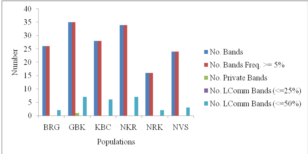
Figure 5: Total band patterns for binary (diploid) data by populations
