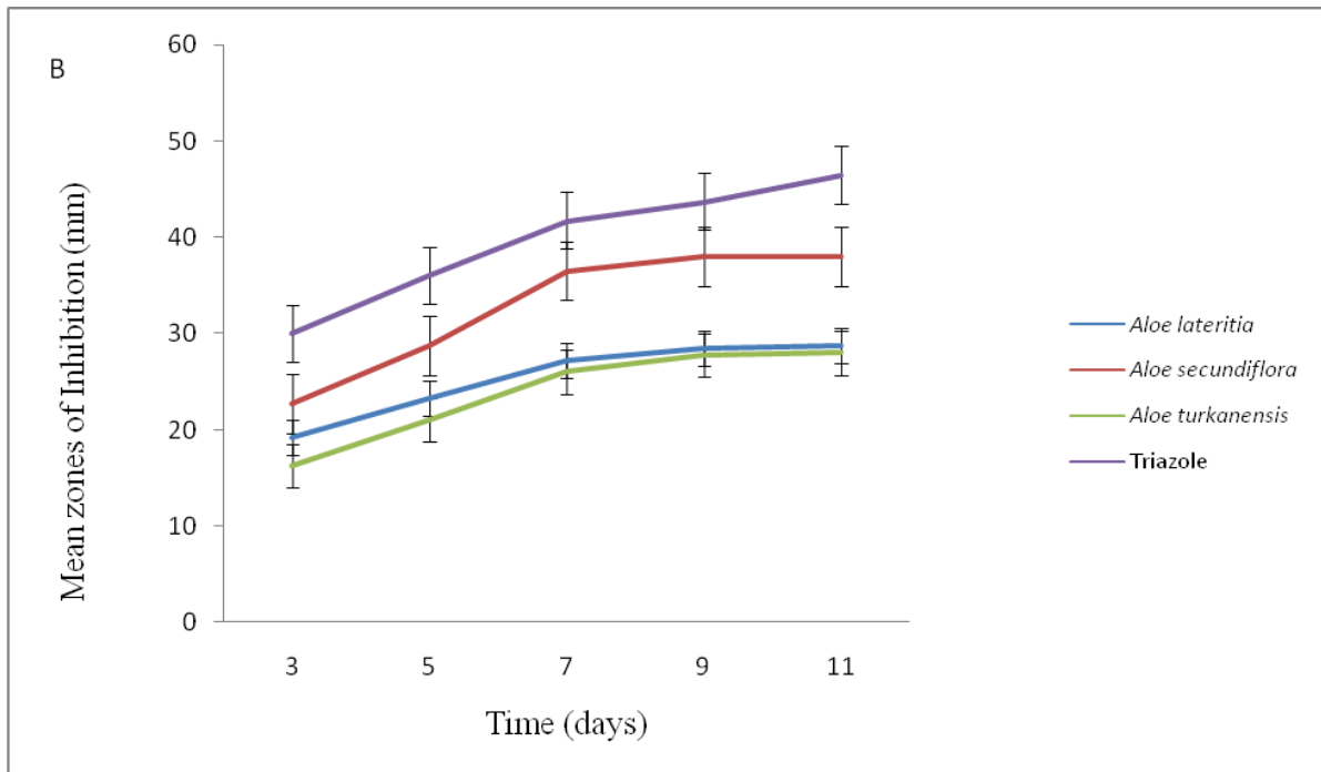
Figure 10: Mean inhibition (mm) of growth of F. oxysporum (A) and P. ultimum (B) by crude extracts of different Aloe species at a 100mg/100 \mu l concentration over time.
